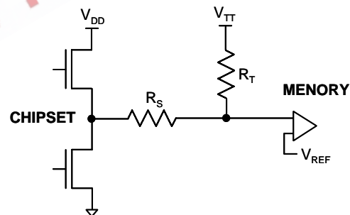
Figure 1. SSTL-Termination Scheme
