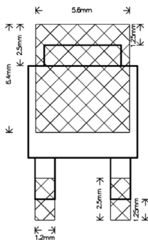
TO-252
