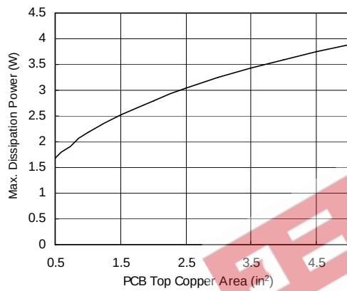
G1084 Max. Power Dissipation vs. PCB Top Copper Area
