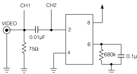
Test Circuit 2
