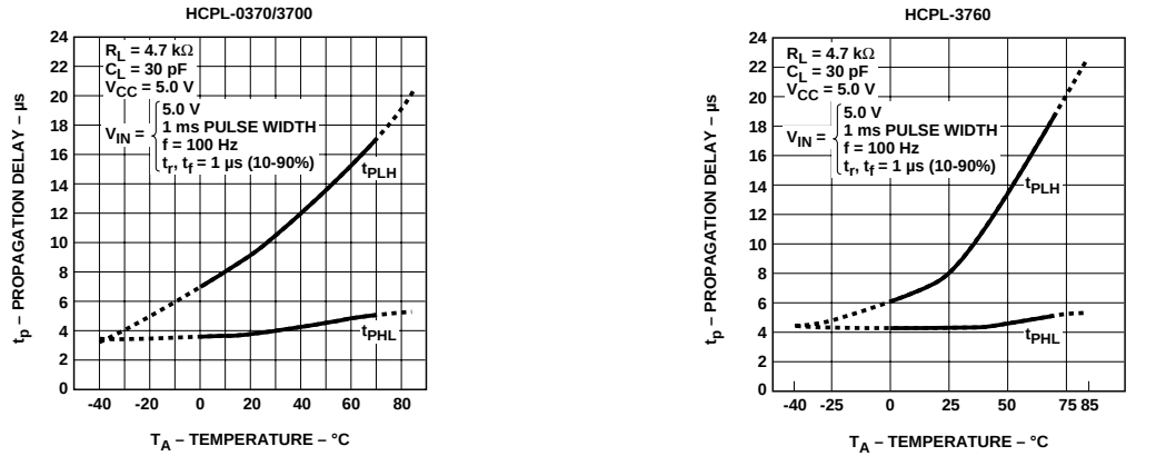
Figure 7. Typical Propagation Delay vs. Temperature.
