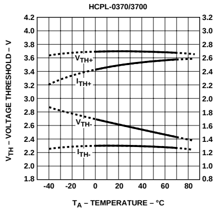
Figure 3. Typical DC Threshold Levels vs. Temperature.
