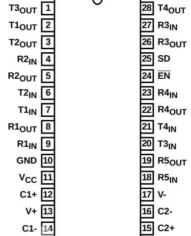
HIN211A (SOIC, SSOP) TOP VIEW
