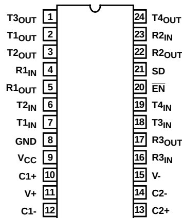
HIN236A (PDIP, SOIC, SSOP) TOP VIEW
