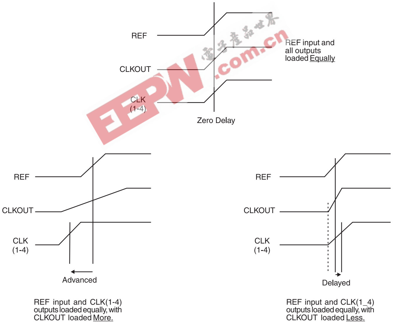
Timing diagrams with different loading configurations
