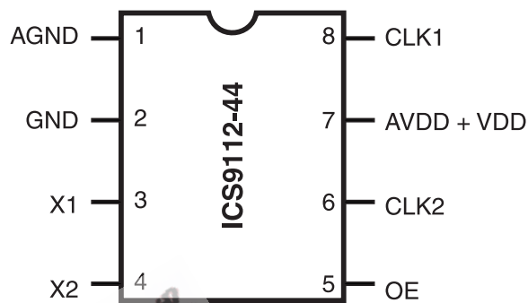
8-Pin SOIC
