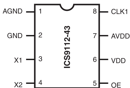
8-Pin SOIC
