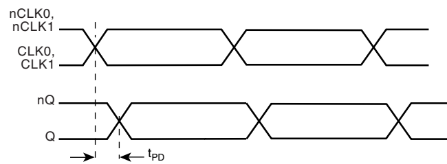
PROPAGATION DELAY
