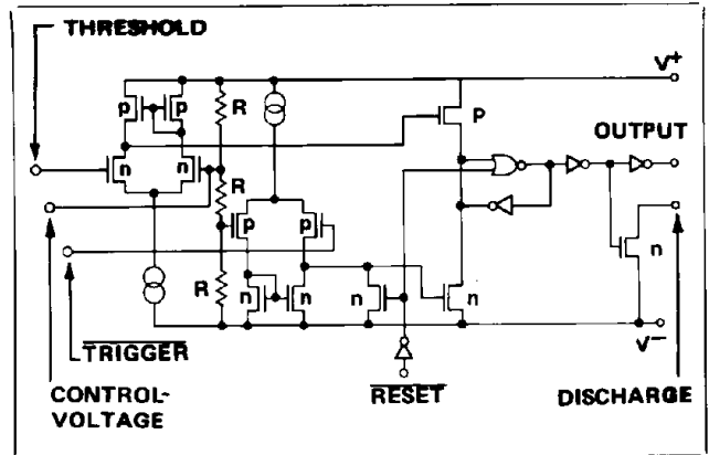
Figure 5. Equivalent circuit.
