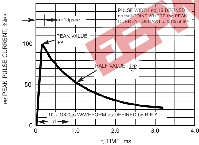
FIG. 3 - PULSE WAVEFORM
