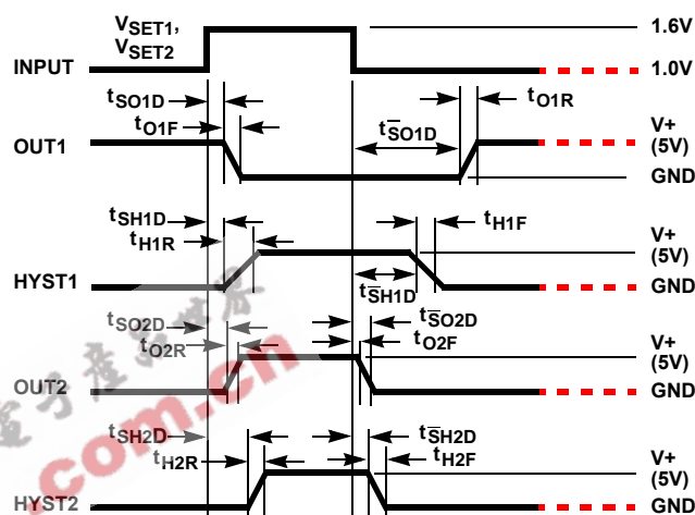
FIGURE 8. SWITCHING WAVEFORMS
