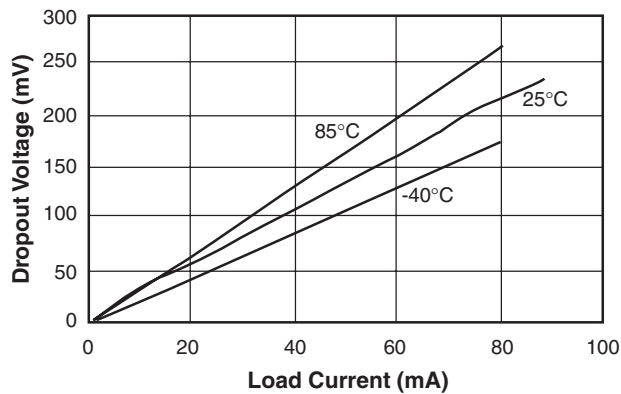
Dropout Voltage
