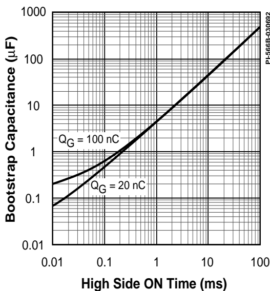
Figure 5. High-side On Time versus Bootstrap Capacitor.
