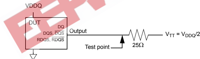
Figure 2 - Slew Rate Test Load
