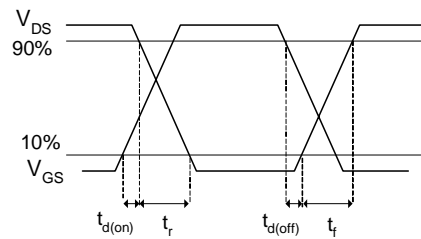
Fig 17. Switching Time Waveforms
