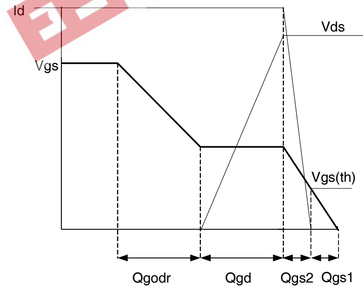
Fig 16. Gate Charge Waveform
