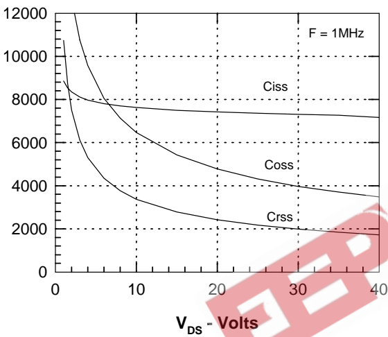
Figure 9. Capacitance Curves
