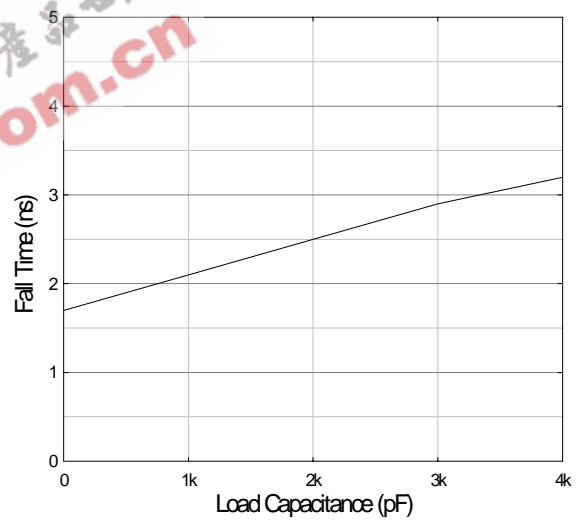
Fig. 4 Fall Time vs. Load Capacitance V_{CC} = 15V, V_{CH} = 12V \text{ To } 2V
