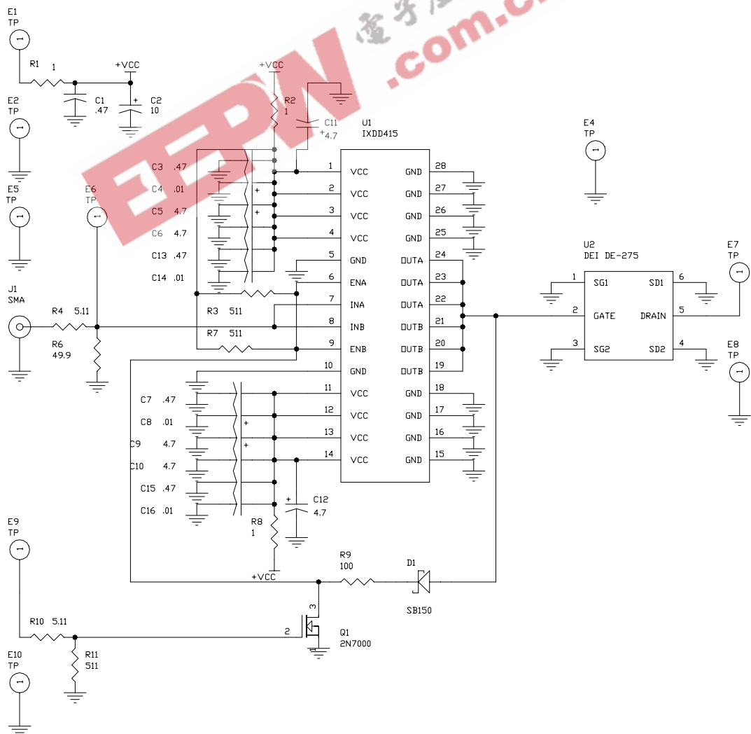
Figure 14 - High Frequency Gate Drive Circuit
