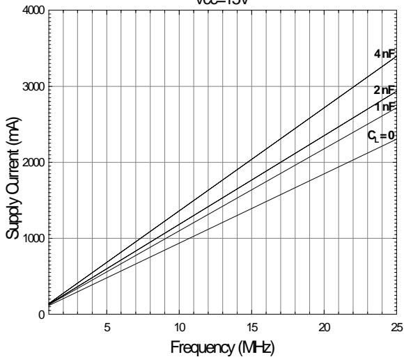
Fig. 5 Supply Current vs. Frequency V_{CC} = 15V
