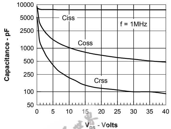
Fig. 8. Capacitance Curves
