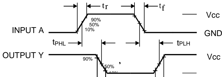
Figure 1. Switching Waveforms
