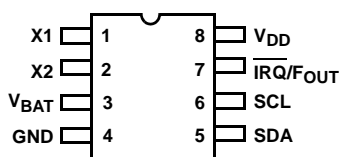
ISL1208 (8 LD MSOP, SOIC) TOP VIEW
