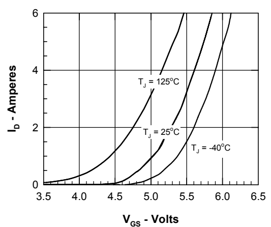
Fig. 6. Admittance Curves
