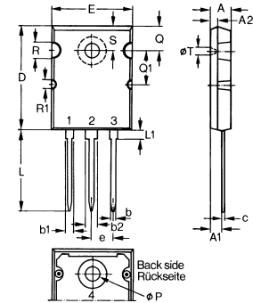
TO-264 AA Outline
