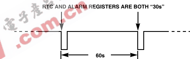
FIGURE 14. \overline{\text{IRQ}}/\text{F}_{\text{OUT}} WAVEFORM
