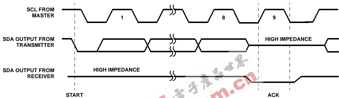
FIGURE 16. ACKNOWLEDGE RESPONSE FROM RECEIVER
