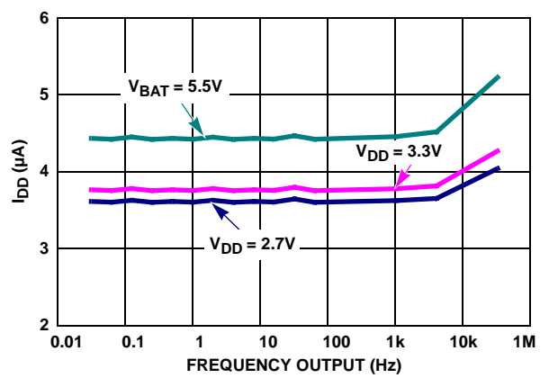
FIGURE 7. F_{OUT} vs I_{DD}
