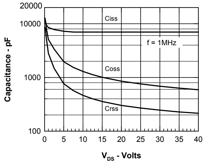
Fig. 7 Capacitance Curves
