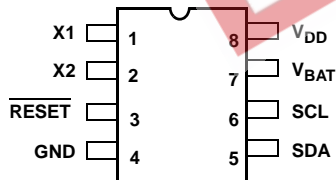
ISL12027 (8 LD SOIC) TOP VIEW
