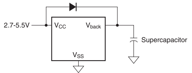
FIGURE 28. SUPERCAPACITOR CHARGING CIRCUIT
