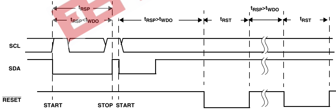
FIGURE 3. WATCHDOG TIMING
