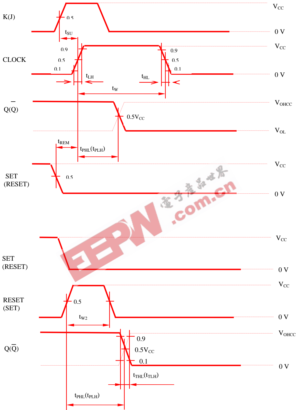
Figure 1. Switching Waveforms
