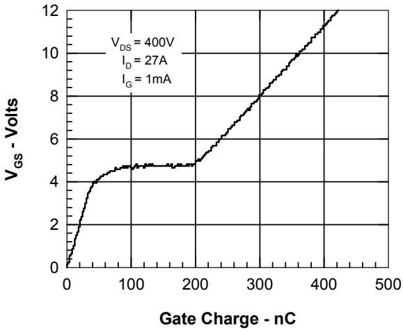
Figure 7. Gate Charge
