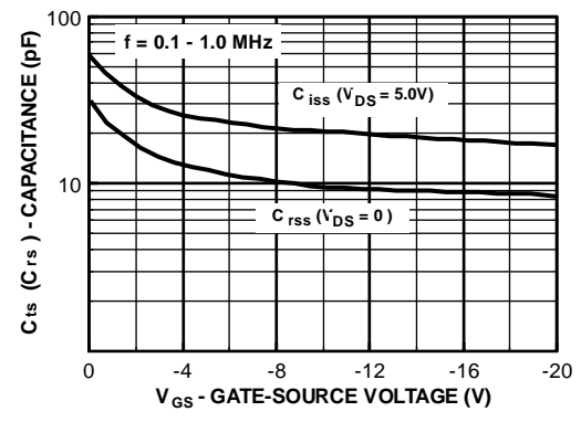
Common Drain-Source
