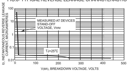
FIG.6- TYPICAL REVERSE LEAKAGE CHARACTERISTICS
