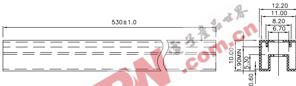
A-A Side view
