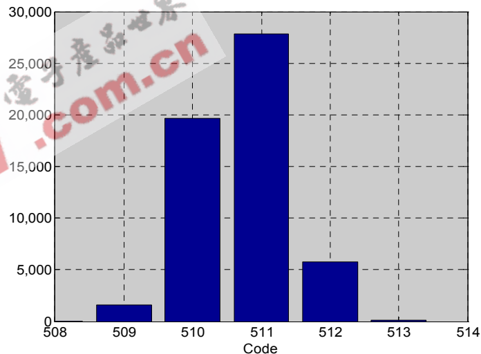
Figure 12. Noise Histogram
