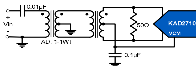
Figure 19. Transformer Input
