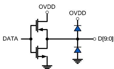
Figure 29. CMOS Outputs
