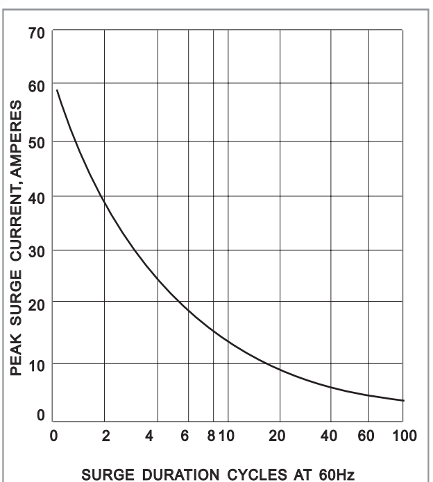
FIG.4-NON-RECURRENT SURGE RATING
