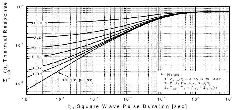
Figure 11. Thermal Response
