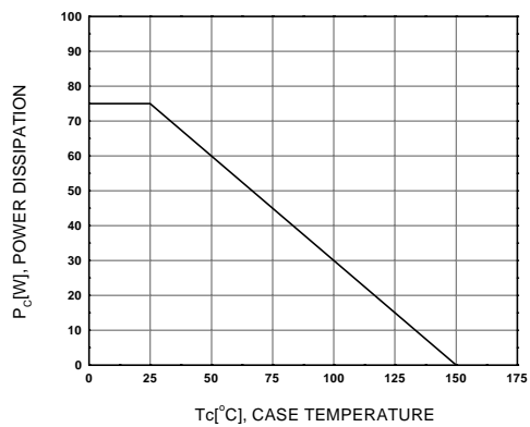
Figure 7. Power Derating
