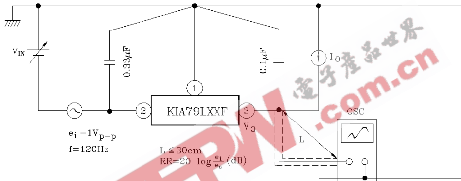
TEST CIRCUIT 2
