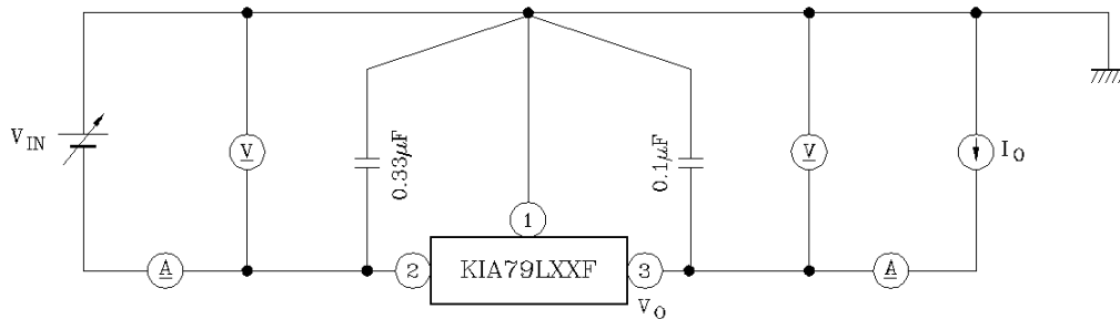
TEST CIRCUIT 1
