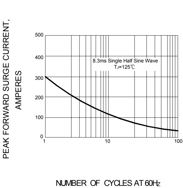
FIG.1 – PEAK FORWARD SURGE CURRENT
