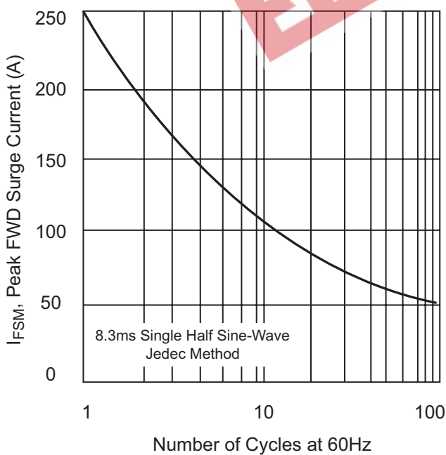
Fig. 3 Max Non-Repetitive FWD Surge Current
