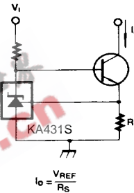
Figure 17. Constant-Current Sink
