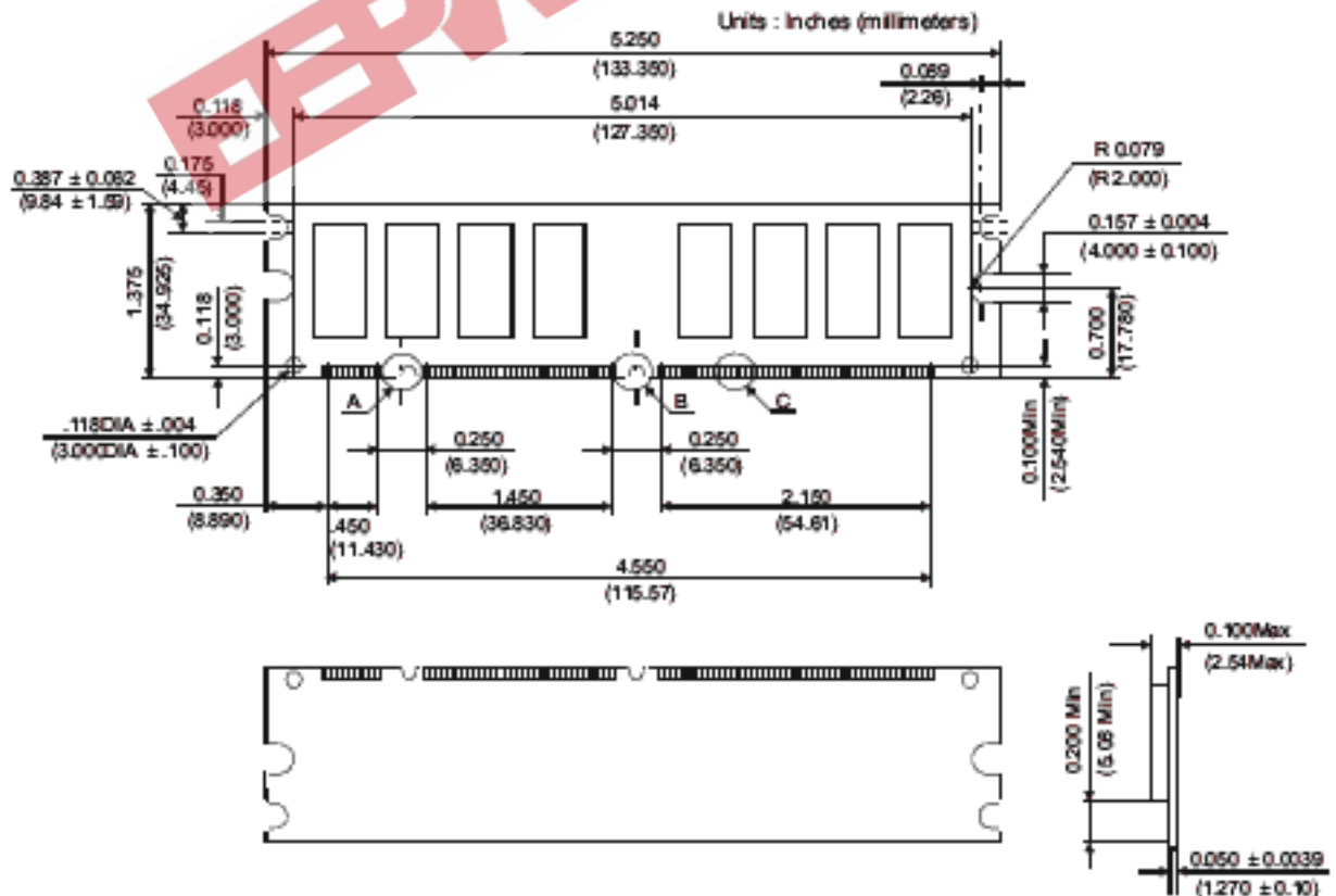
Figure 1: KVR100X64C3/64 168-Pin SDRAM Module
