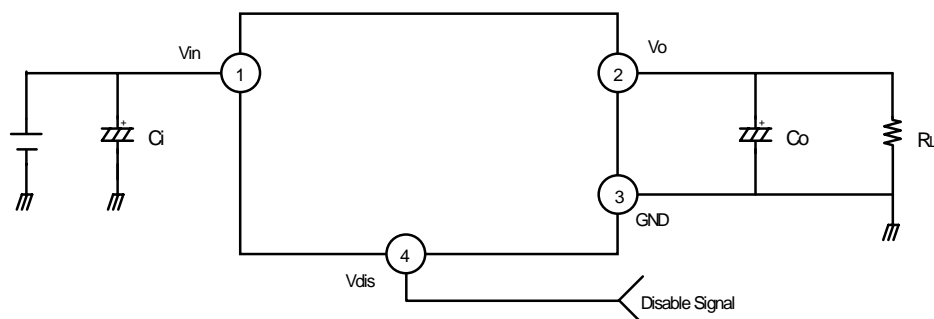
Figure 1. Application Circuit
