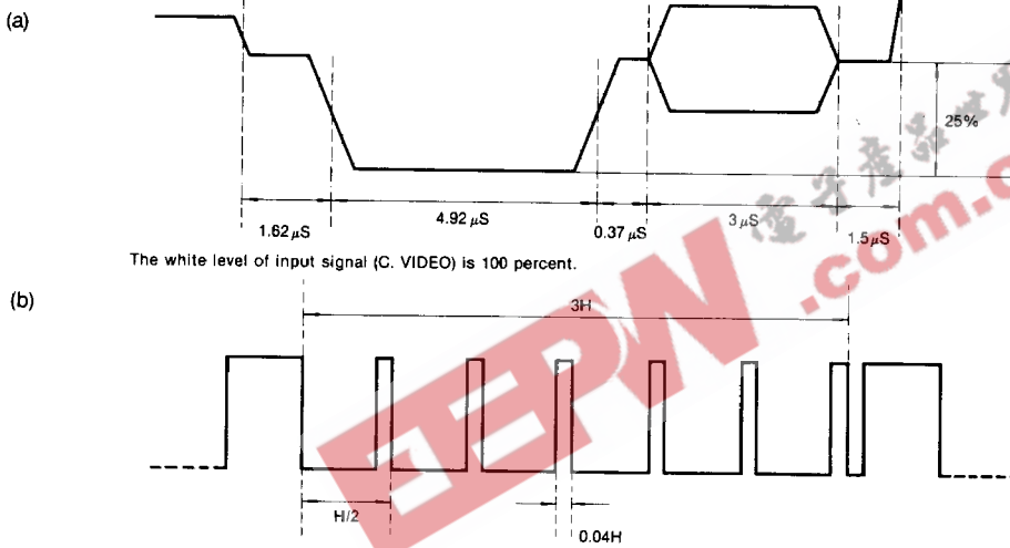
Fig. 3 2V_{pp} Positive composite video signal (a) Horizontal sync pulse. (b) Vertical sync pulse. H equals 63.5 \mu s .
