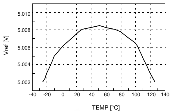
Figure 4. Bandgap Reference Voltage
