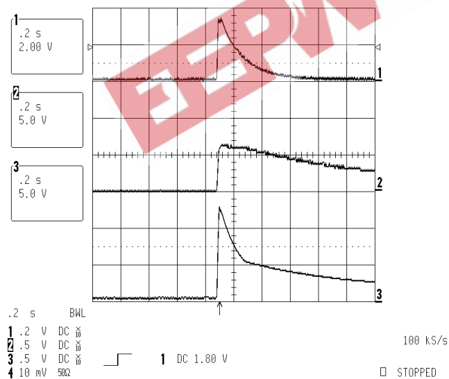
Figure 26. No Load Protection
