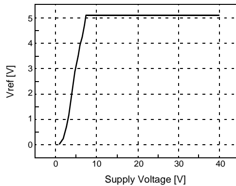
Figure 22. Reference Voltage
