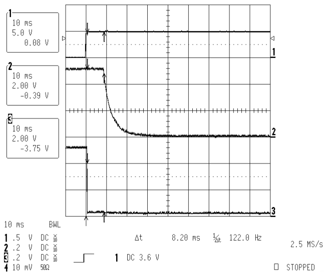
Figure 25. Power Down Warning
