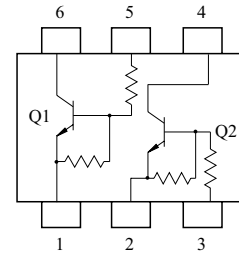
EQUIVALENT CIRCUIT (TOP VIEW)
