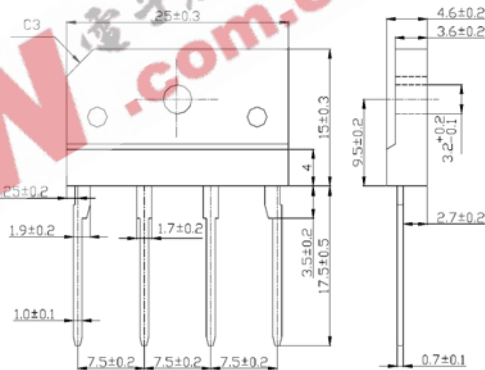
Package outline dimensions in millimeters
