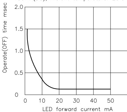
LED forward current vs. operate(OFF) time Across terminals 5,7 and 6,8 pin; Load voltage: 400V(DC); Continuous load current: 130mA(DC); Ambient temperature: 25°C
