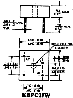
KBPC25W
