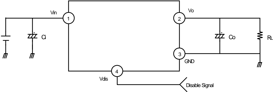
Figure 1. Application Circuit
