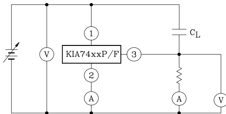
TEST CIRCUIT 1.
